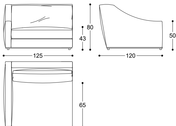
Article: Terminal element 125 x 120 Left Code: SX-MAR3F Article: Terminal element 125 x 120 Right Code: DX-MAR3E
