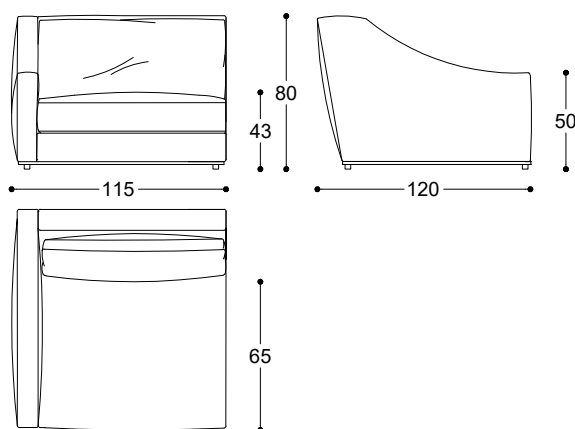
Article: Terminal element 115 x 120 Left Code: SX-MAR2D Article: Terminal element 115x 120 Right Code: DX-MAR2C
