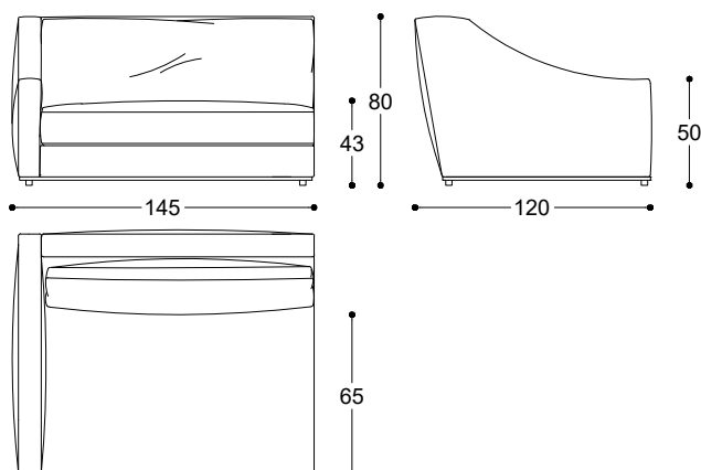
Article: Terminal element 145 x 120 Left Code: SX-MAR5H Article: Terminal element 145 x 120 Right Code: DX-MAR5G
