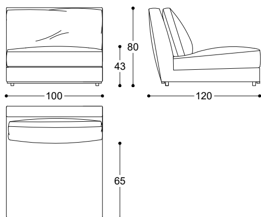
Article: Linear element 100 x 120 Code: MAR20
